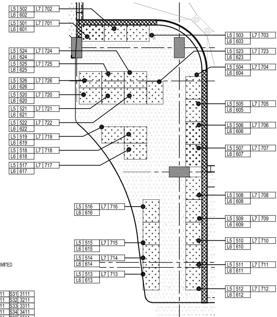
PARKING STRUCTURE STORAGE LEVELS 5, 6, 7
