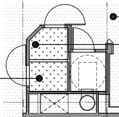
TOWER STORAGE LEVELS 9 THROUGH 41
